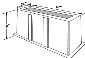
ELECTRICAL SWITCH MOLE CABINET BASE DETAIL
